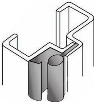
Dual Contact Thermal Break Weather Seal
