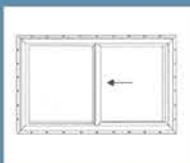
HORIZONTAL SLIDERS 1200 SERIES Width = 24" to 96" | Height = 14" to 64"
